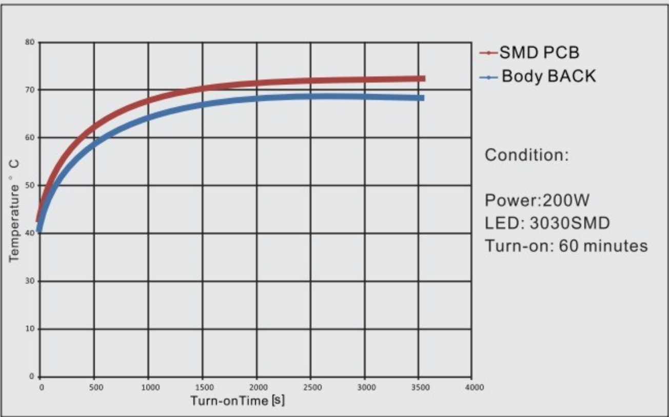
Temperature Rise Curve
