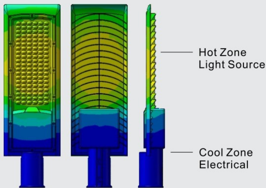
Thermal Conductivity
