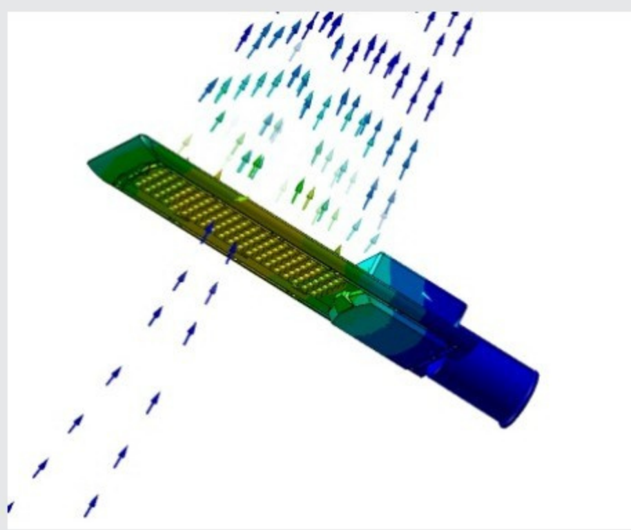
Thermal Air Convection
